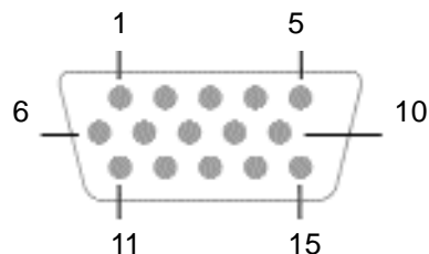
VGA CONNECTOR
